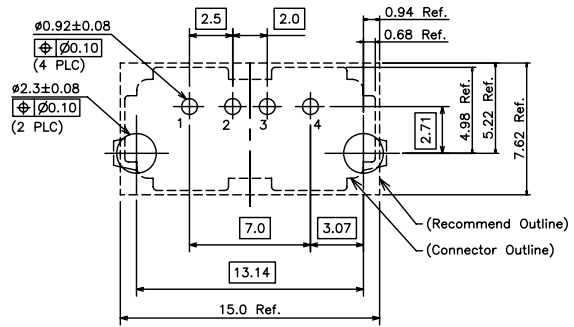
RECOMMENDED P.C.BOARD LAYOUT(T=1.6) (TOP VIEW)(TOLERANCE:±0.05)
