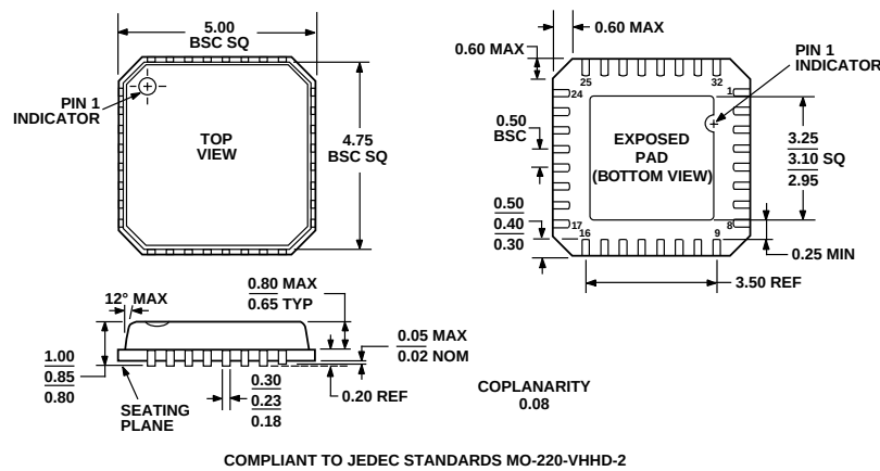
Figure 64. 32-Lead Lead Frame Chip Scale Package [LFCSP] 5 mm × 5 mm Body (CP-32-2) Dimensions shown in millimeters
