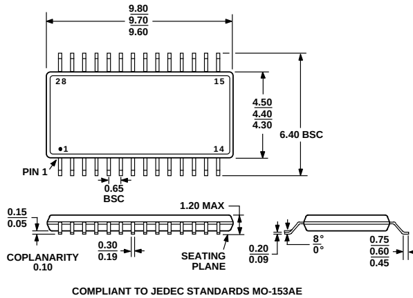
Figure 63. 28-Lead Thin Shrink Small Outline Package [TSSOP] (RU-28) Dimensions shown in millimeters
