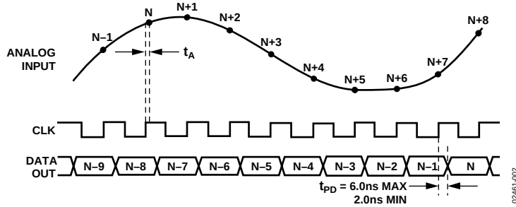
Figure 2. Timing Diagram
