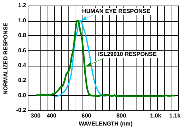
FIGURE 7. SPECTRAL RESPONSE
