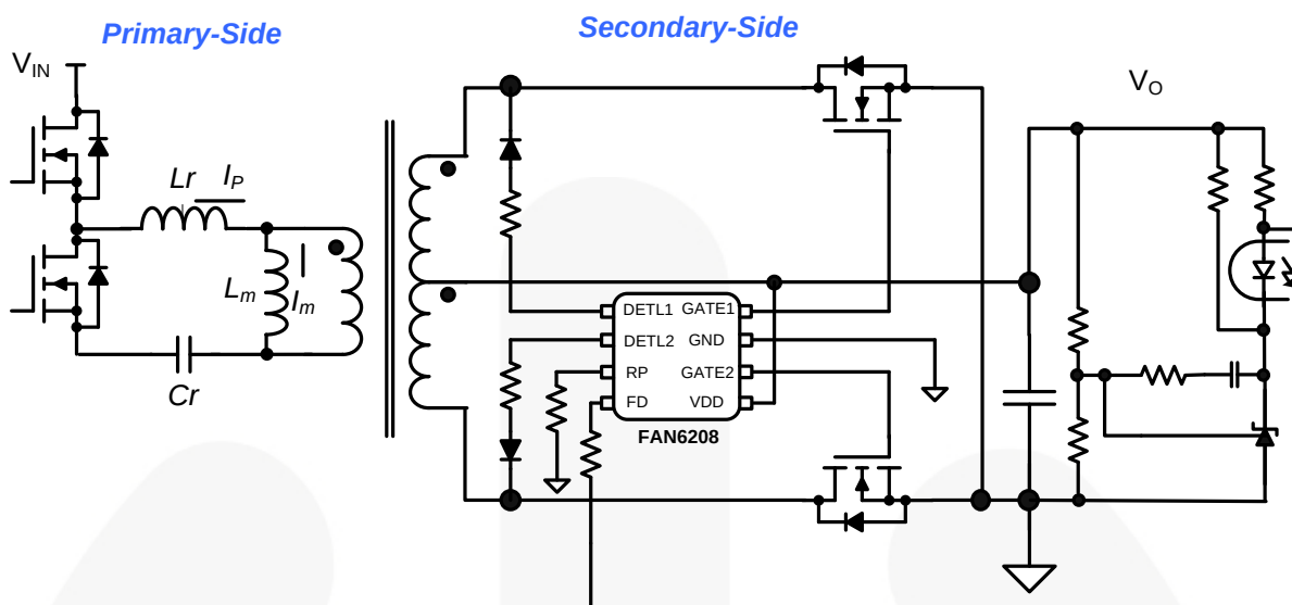
Figure 1. Typical Application
