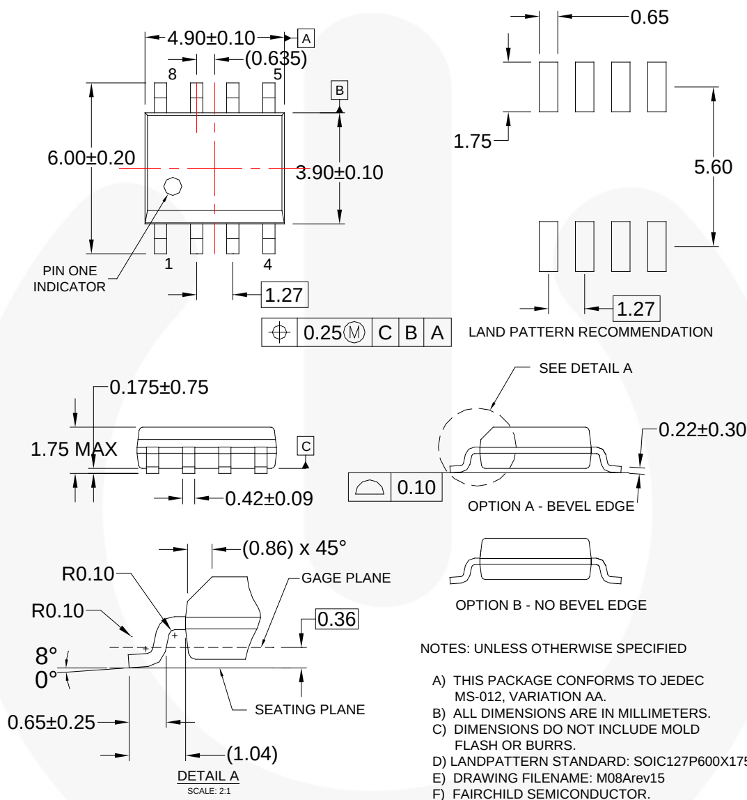
Figure 45. 8-Lead, SOIC, JEDEC MS-012, .150-Inch Narrow Body
