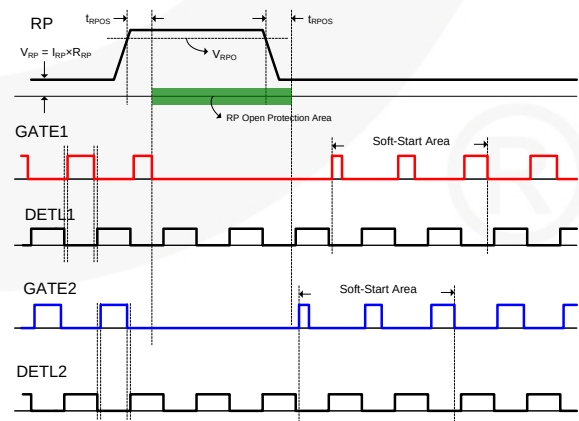
Figure 18. RP Pin Open Protection
