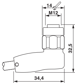
Dimensioned drawing
