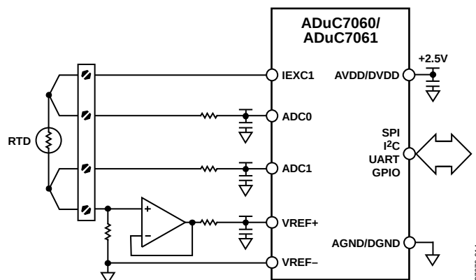
Figure 20. Example of an RTD Interface Circuit
