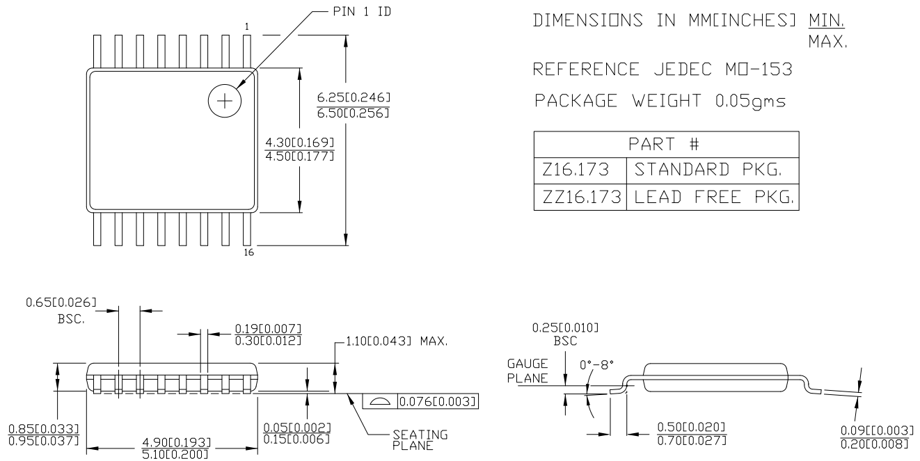
Figure 8. 16-pin TSSOP 4.40 mm Body ZZ16
