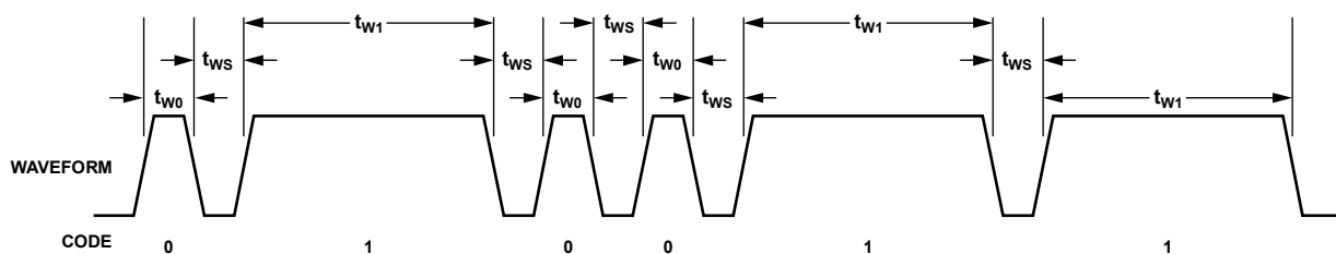
Figure 49. Timing Diagram for Code 010011
