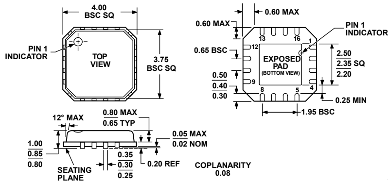
Figure 57. 16-Lead Lead Frame Chip Scale Package [LFCSP_VQ] 4 mm x 4 mm Body, Very Thin Quad (CP-16-10) Dimensions shown in millimeters
