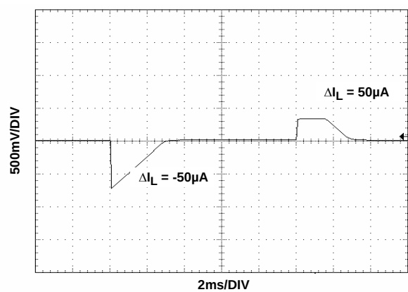
FIGURE 65. LOAD TRANSIENT RESPONSE
