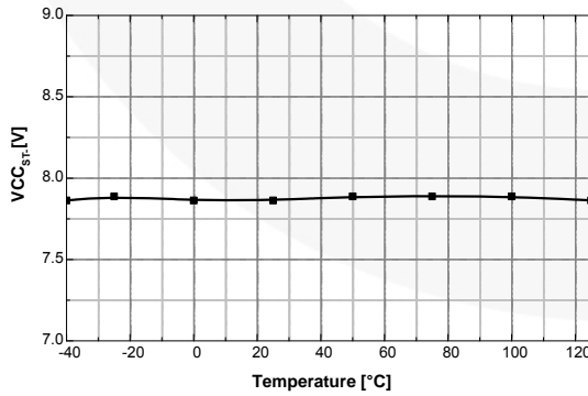
Figure 17. V CCS- vs. Temperature
