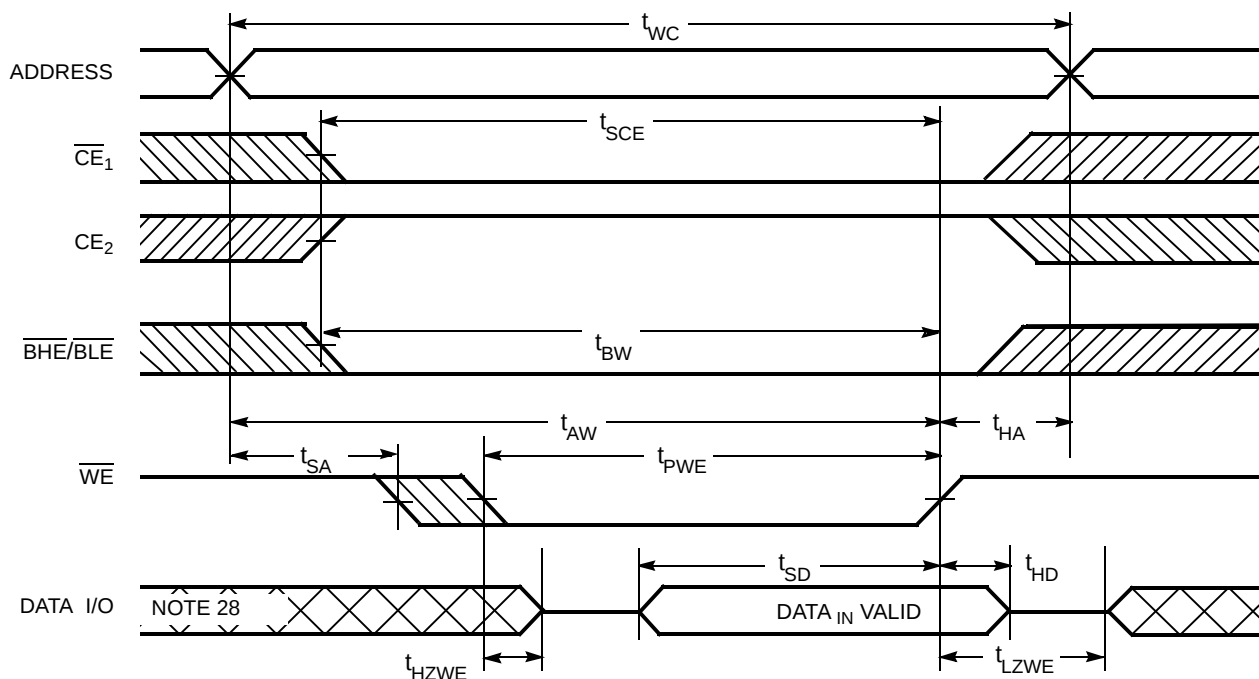
Figure 9. Write Cycle 4 ( \overline{\text{BHE/BLE}} Controlled, \overline{\text{OE}} LOW) [27, 28]
