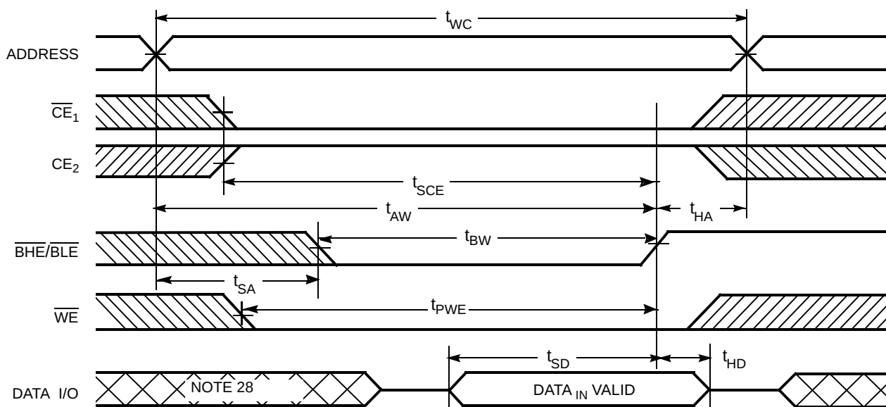
Figure 9. Write Cycle 4 ( \overline{\text{BHE/BLE}} Controlled, \overline{\text{OE}} LOW) [27, 28]
