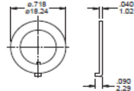
Locking ring supplied with B13,B18,B20 bushing
