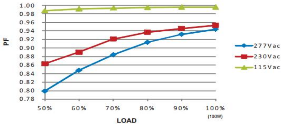
Constant Current Mode
