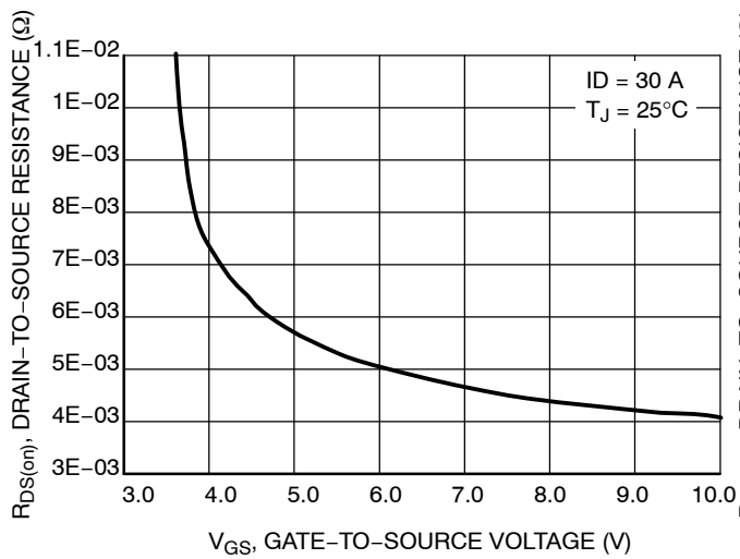
Figure 3. On-Region versus V_{GS}
