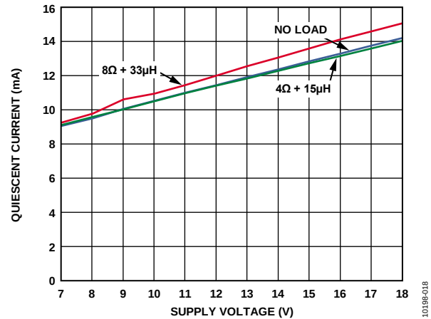
Figure 18. Quiescent Current vs. Supply Voltage, R_L = 8\Omega + 33\mu\text{H} , No Load, R_L = 4\Omega + 15\mu\text{H}
