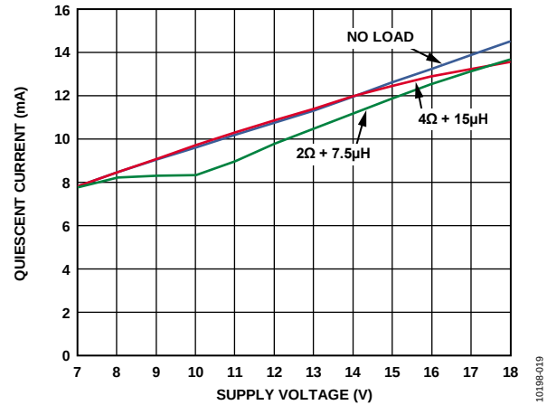
Figure 19. Quiescent Current vs. Supply Voltage, Mono Mode, No Load, R_L = 4\Omega + 15\mu\text{H} , R_L = 2\Omega + 7.5\mu\text{H}
