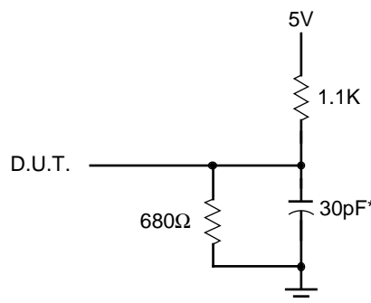
Figure 1. Output Load
