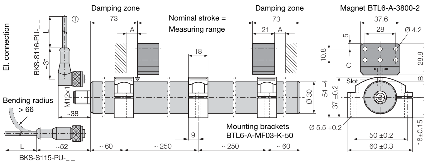
Fig. 3-1: Dimensional drawing (BTL6...A1-S115 transducer with floating magnet BTL6-A-3800-2 and mounting brackets BTL6-A-MF03-K-50)
