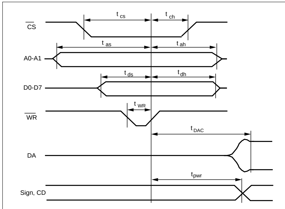
Figure 11. Timing
