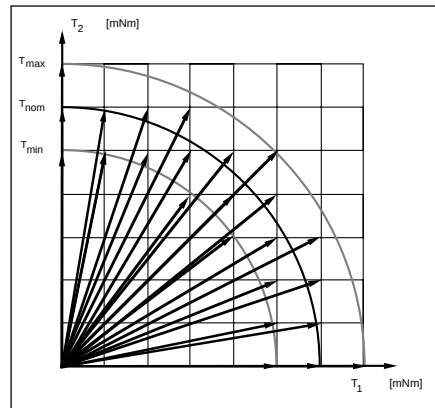
Figure 6b. An example of accessible positions with a given torque deviation/fullstep. Note that 1:st µstep sets highest resolution. Data points are exaggerated for illustration purpose.
