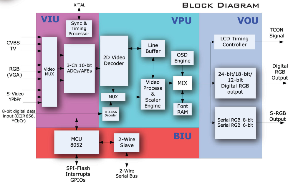
BLOCK DIAGRAM
