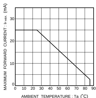
Fig. 31 Maximum forward current vs. ambient temperature
