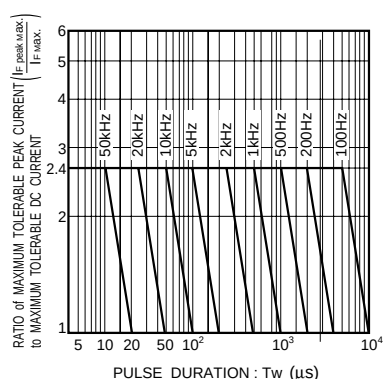
Fig. 29 Maximum tolerable peak current vs. pulse duration
