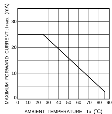
Fig. 25 Maximum forward current vs. ambient temperature
