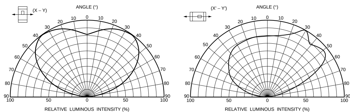
Fig.1 Directional pattern
