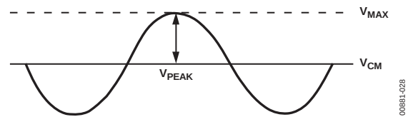
Figure 28. Common-Mode Definition
