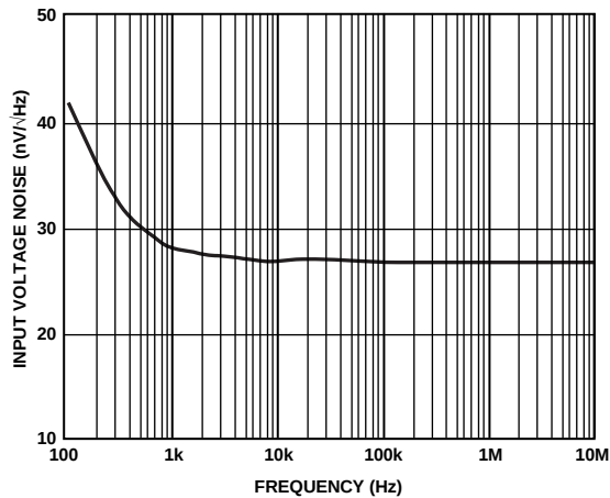
Figure 14. Noise Spectral Density
