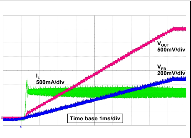
Figure 31. Soft-start
