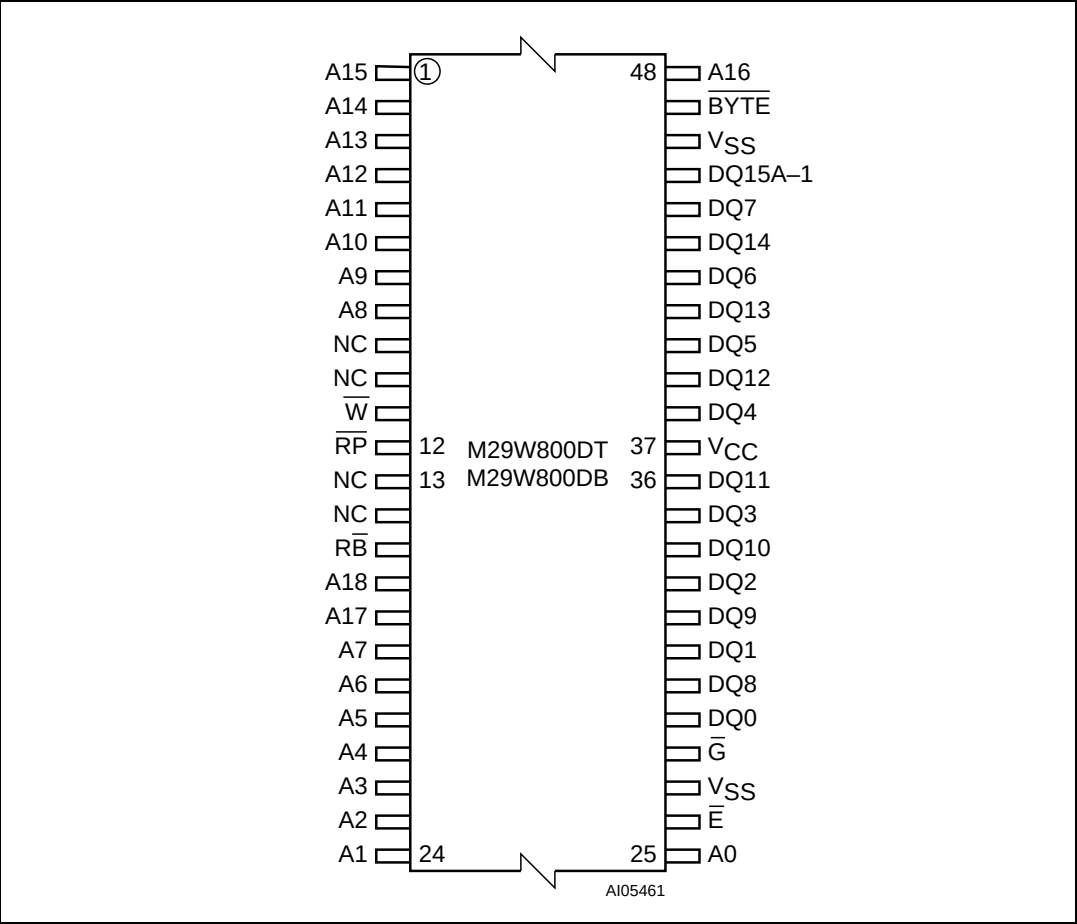
Figure 3. TSOP Connections
