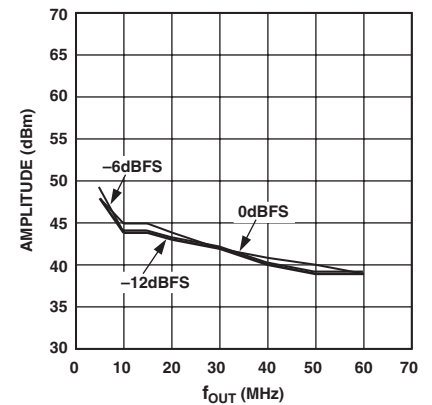
TPC 9. Out-of-Band SFDR vs. f_{OUT} @ f_{DATA} = 160 MSPS
