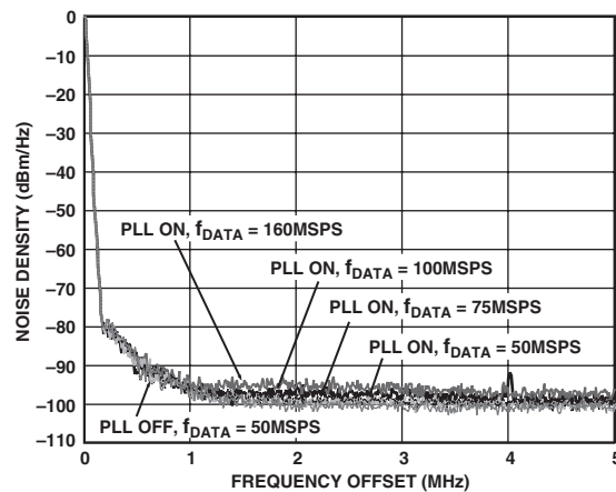
Figure 9. Phase Noise of PLL Clock Multiplier at Exact f_{\text{OUT}} = f_{\text{DATA}}/4 at Different f_{\text{DATA}} Settings with Optimum DIV0/DIV1 Settings Using R & S FSEA30, RBW = 30 kHz
