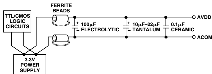
Figure 29. Differential LC Filter for 3.3 V
