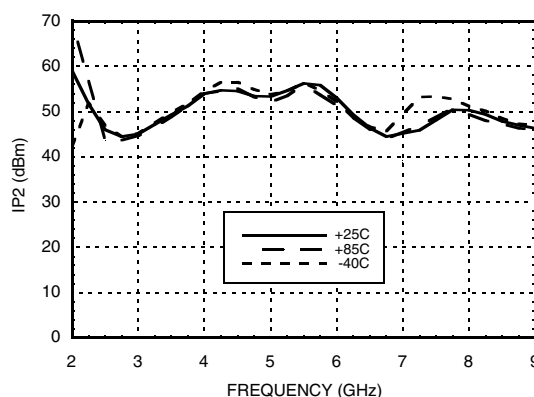
Input IP2 vs. Temperature @ LO = +15 dBm *
