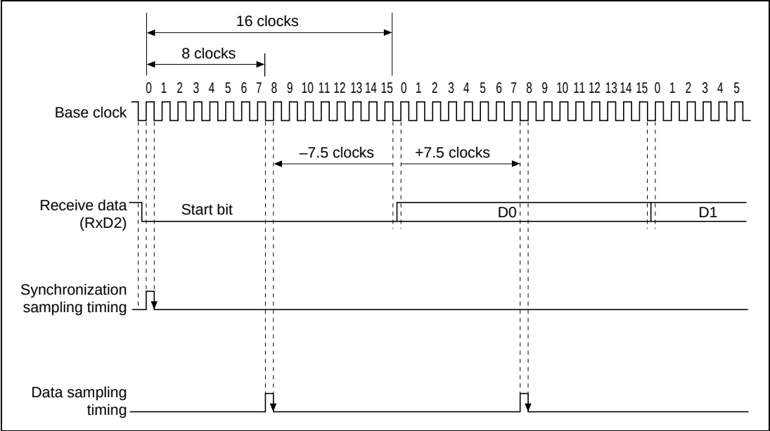
Figure 16.14 Receive Data Sampling Timing in Asynchronous Mode
