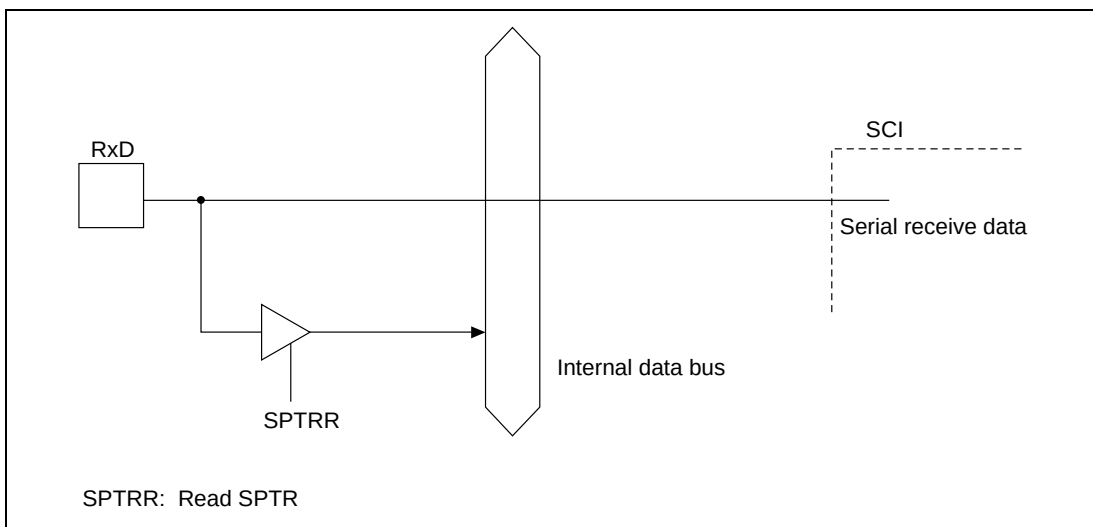
Figure 15.4 RxD Pin
