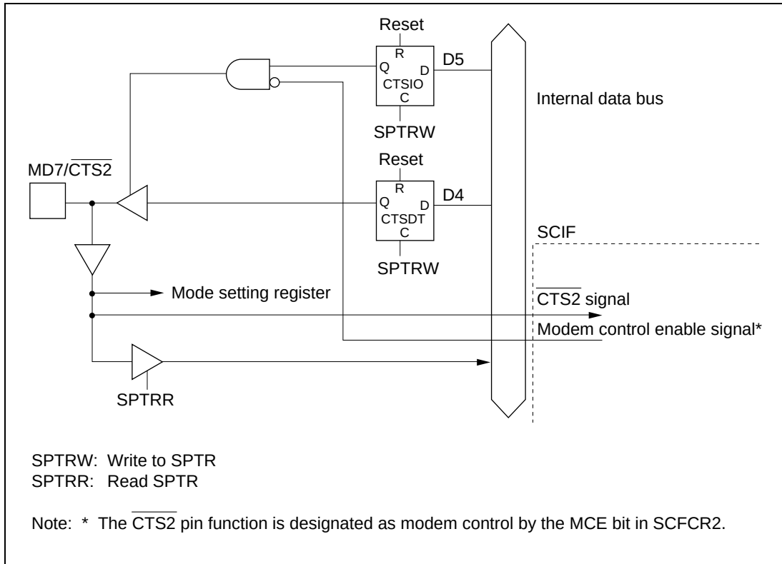
Figure 16.3 MD7/CTS2 Pin
