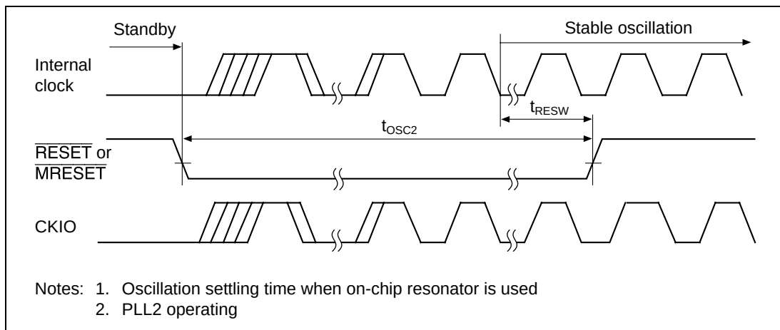
Figure 23.6 Standby Return Oscillation Settling Time (Return by \overline{RESET} or \overline{MRESET} )
