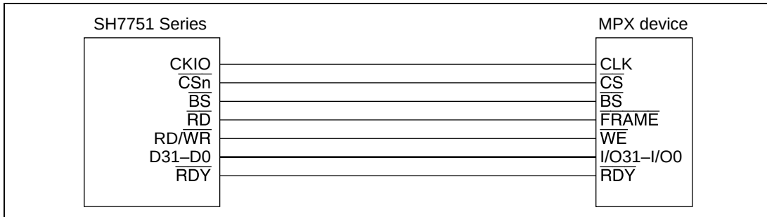
Figure 13.51 Example of 32-Bit Data Width MPX Connection
