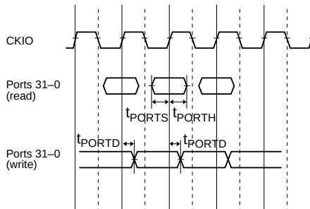
Figure 23.63 I/O Port Input/Output Timing
