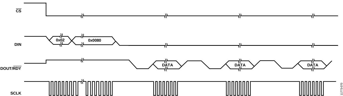
Figure 70. Continuous Read Mode
