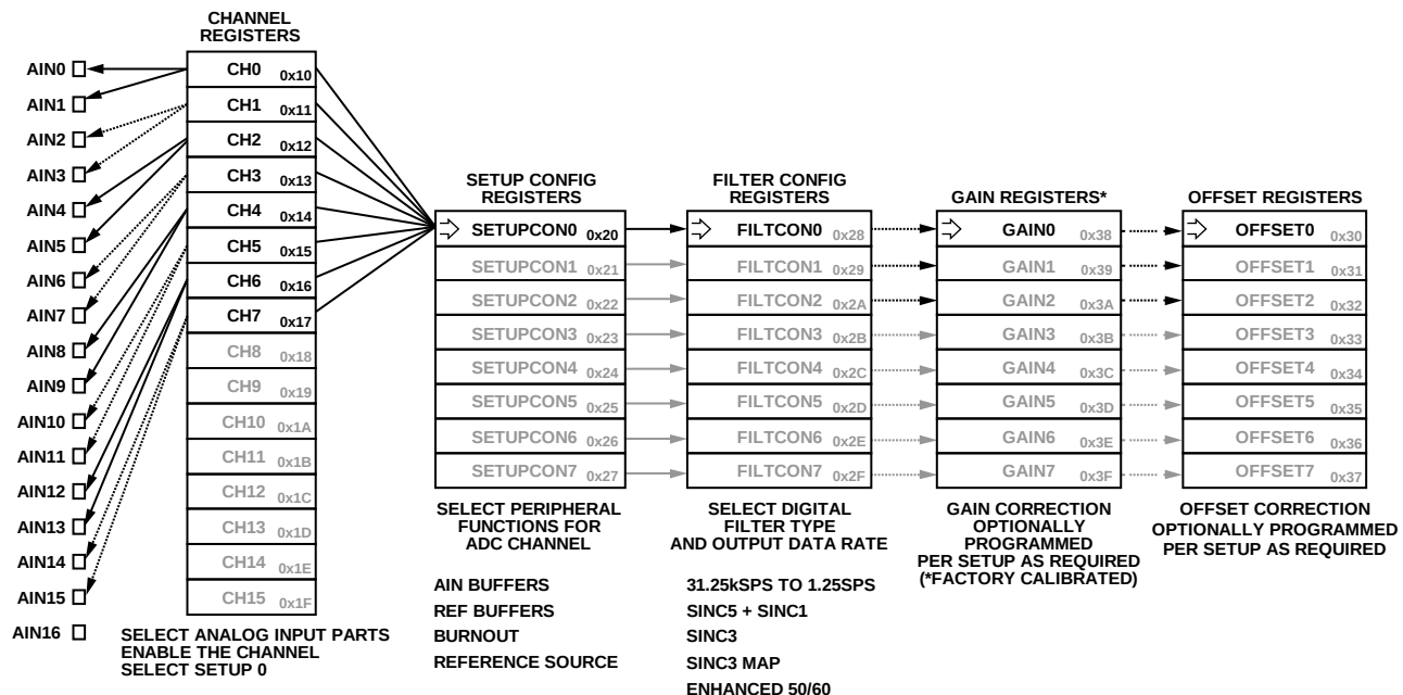
Figure 46. Eight Fully Differential Inputs, All Using a Single Setup (SETUPCON0; FILTERCON0; GAIN0; OFFSET0)
