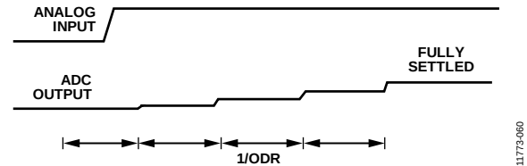
Figure 60. Step Input Without Single Cycle Settling
