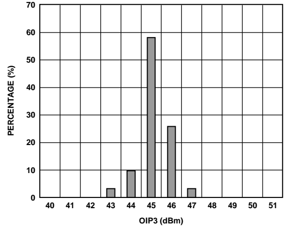
Figure 12. OIP3 Distribution at 190 MHz, P_{OUT} = 3 \text{ dBm}
