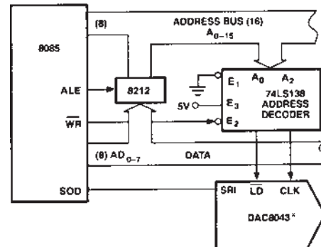
Figure 11. DAC8043 to 8085 Interface
