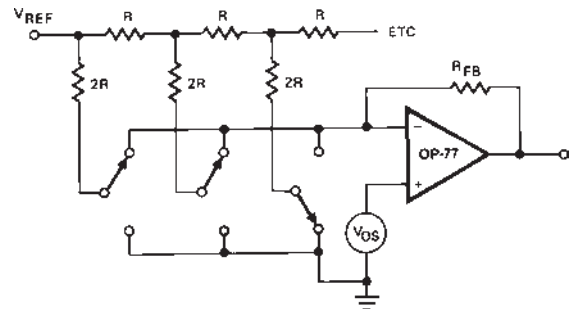
Figure 5. Simplified Circuit
