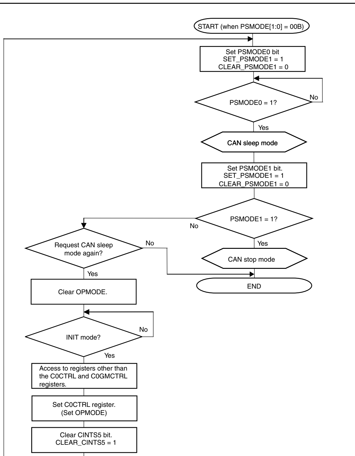
Figure 20-52. Setting CAN Sleep Mode/Stop Mode
