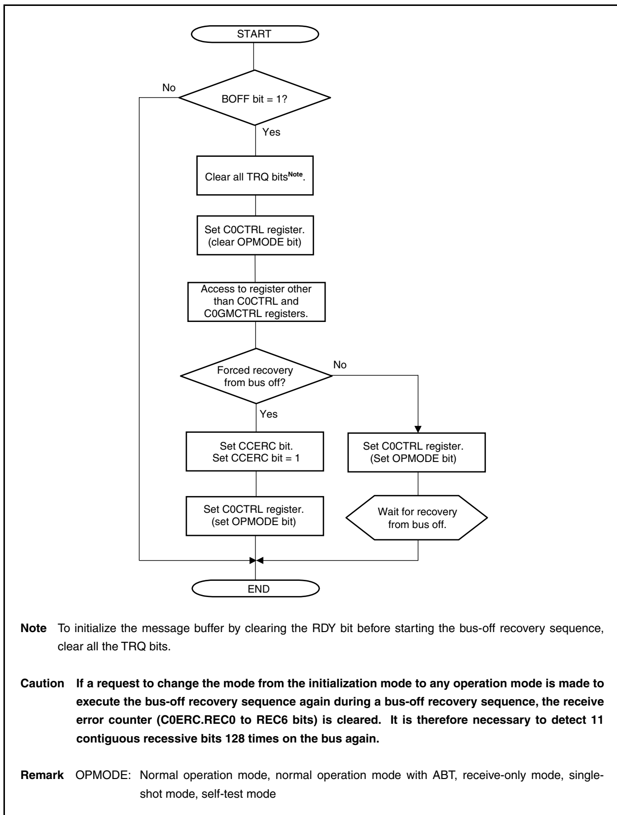
Figure 20-54. Bus-off Recovery (Other Than in Normal Operation Mode with ABT)
