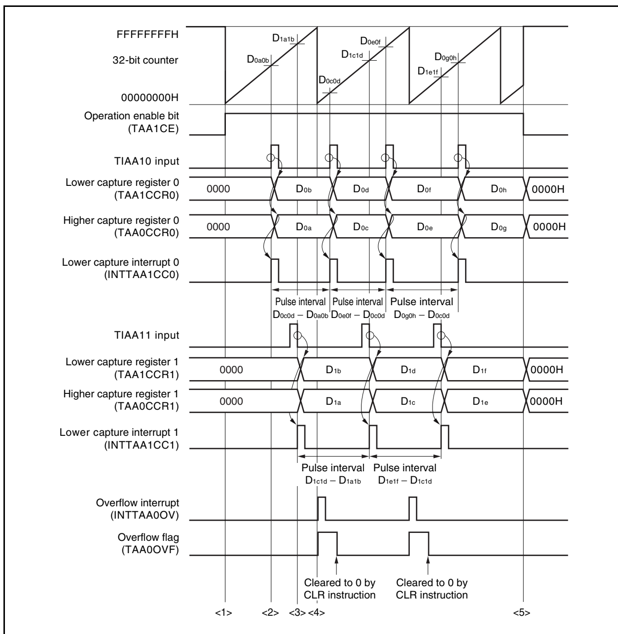
Figure 7-51. Operation Flow in Cascade Connection of TAA1 and TAA0 (1/2)
