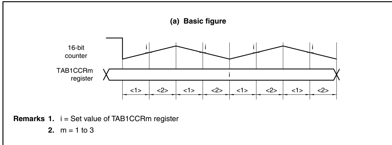
Figure 11-23. Basic Operation of 16-Bit Counter and TAB1CCRMm Register
