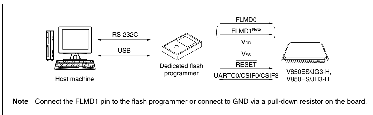
Figure 31-2. Environment Required for Writing Programs to Flash Memory
