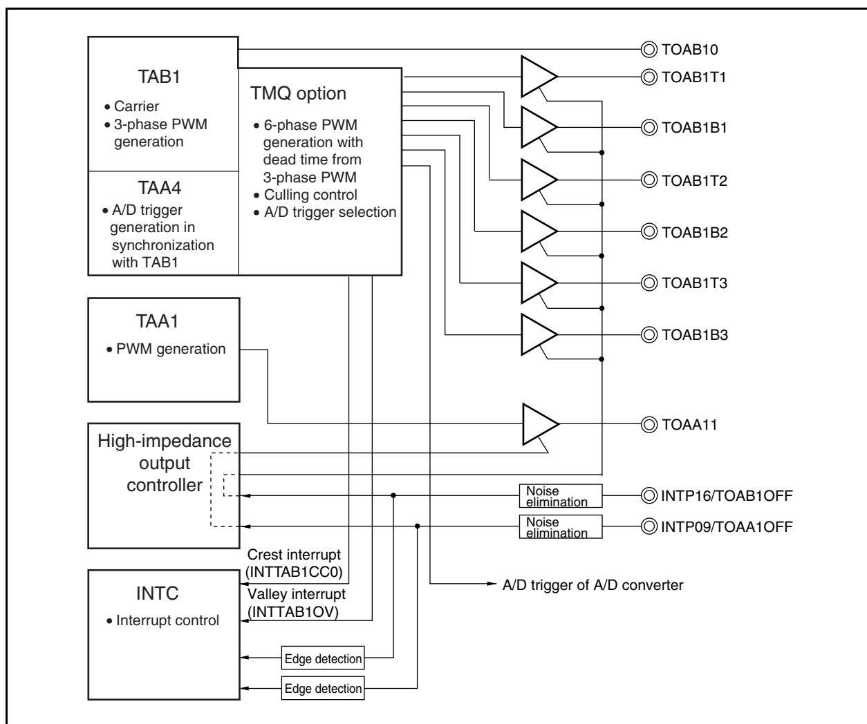
Figure 11-1. Block Diagram of Motor Control
