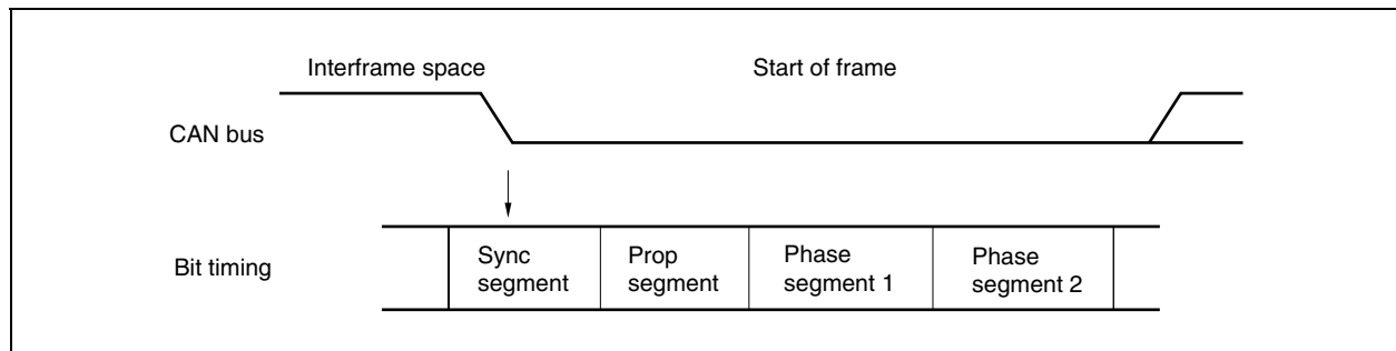
Figure 20-20. Hardware Synchronization Due to Dominant Level Detection During Bus Idle
