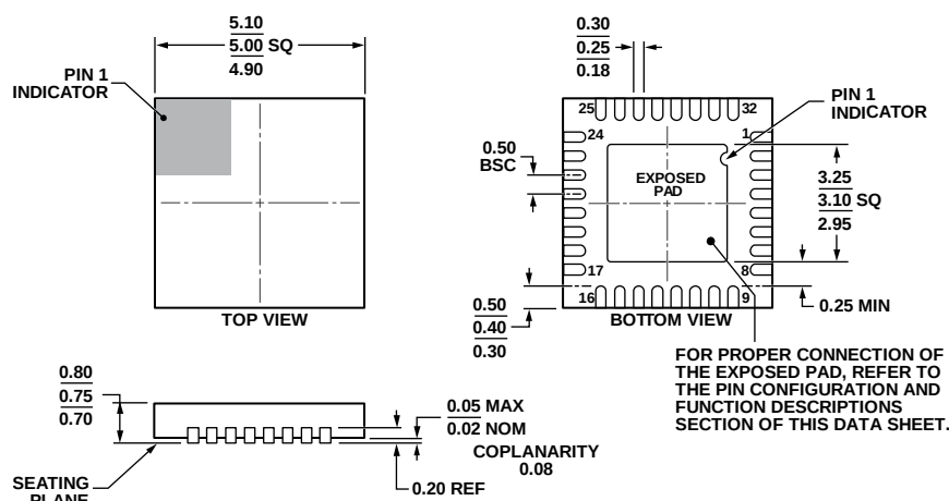
Figure 22. 32-Lead Frame Chip Scale Package [LFCSP_WQ] 5 mm × 5 mm Body, Very Very Thin Quad (CP-32-7)
