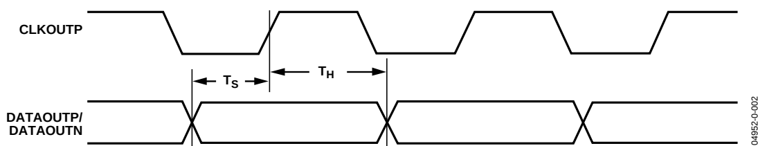
Figure 2. Output Timing
