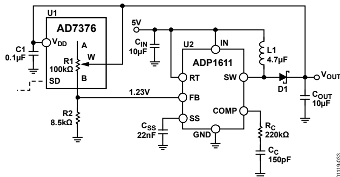
Figure 33. Programmable Power Supply
