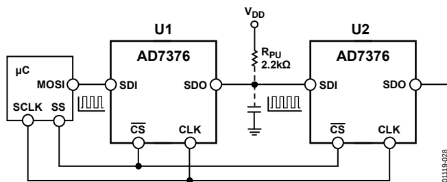
Figure 28. Daisy-Chain Configuration
