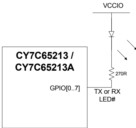
Figure 11. Single-LED Configuration
