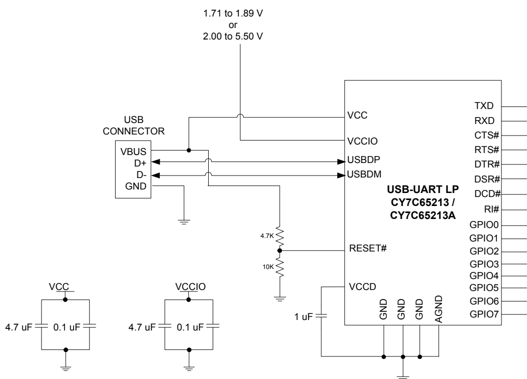
Figure 2. Self-Powered Configuration
