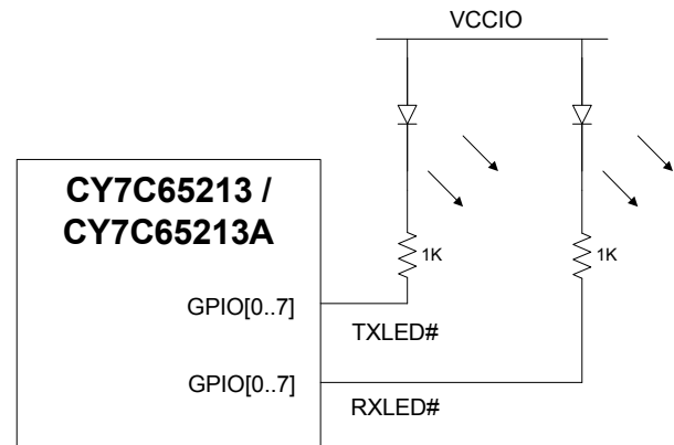
Figure 12. Double-LED Configuration
