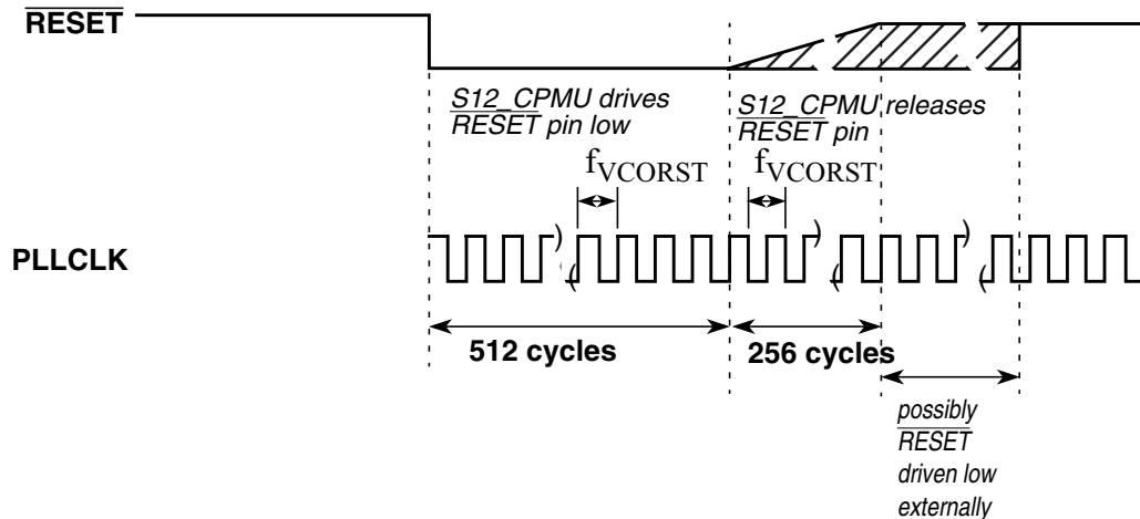
Figure 10-34. RESET Timing
