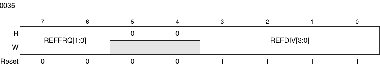
Figure 10-5. S12CPMU Reference Divider Register (CPMUREFDIV)
