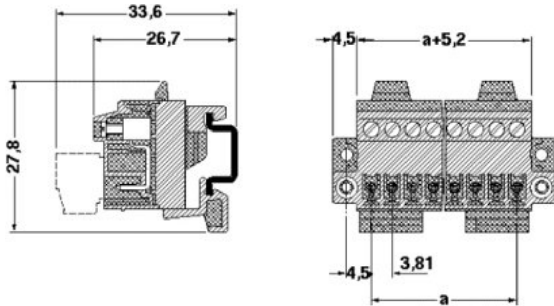
Dimensioned drawing
