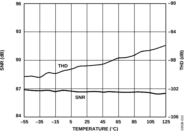
Figure 10. SNR, THD vs. Temperature
