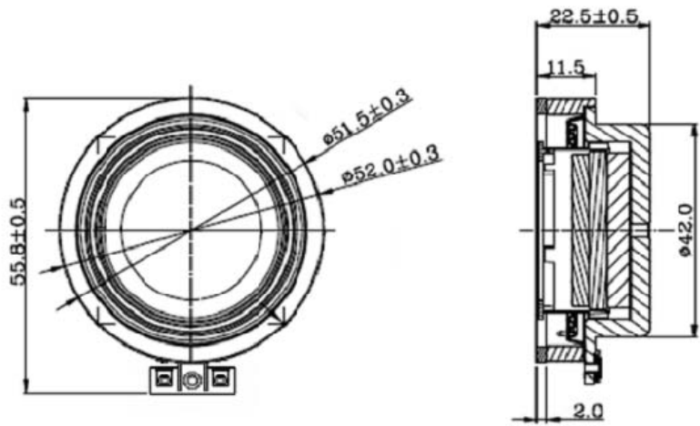
Figure 2.Nominal dimensions.
