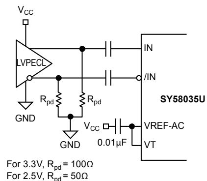
Figure 3b. LVPECL Interface (AC-Coupled)
