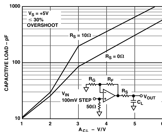
Figure 13. AD8054 Capacitive Load Drive vs. Closed-Loop Gain
