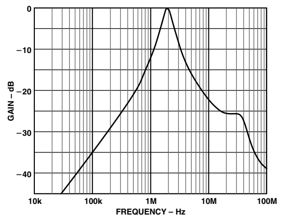
Figure 16. Frequency Response of 2\text{ MHz} Band-Pass Biquad Filter
