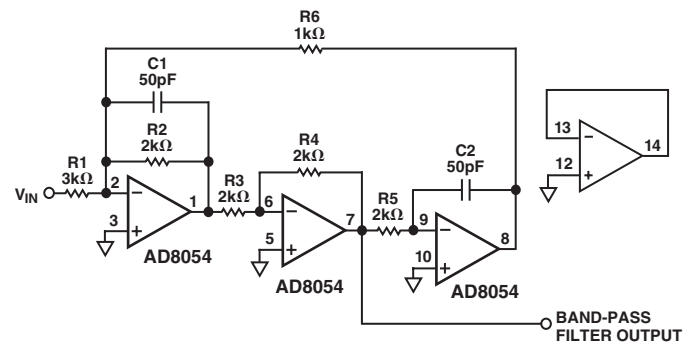
Figure 15. 2\text{ MHz} Biquad Band-Pass Filter Using AD8054
