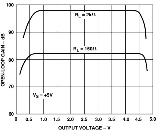
TPC 26. Open-Loop Gain vs. Output Voltage
