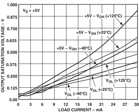
TPC 27. AD8054 Output Saturation Voltage vs. Load Current
