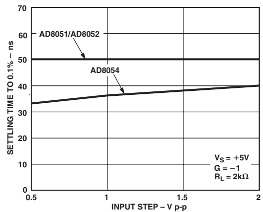
TPC 24. Settling Time vs. Input Step
