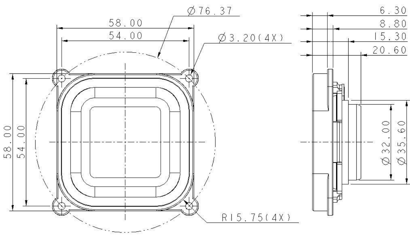
Figure 2. Nominal dimensions
