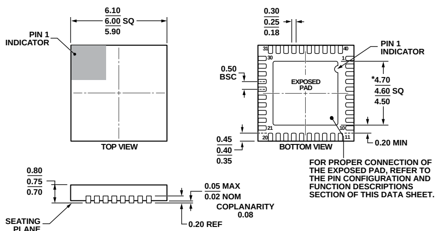
Figure 49. 40-Lead Lead Frame Chip Scale Package [LFCSP_WQ]
