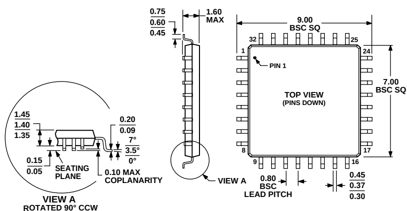
Figure 48. 32-Lead Low Profile Quad Flat Package [LQFP]
