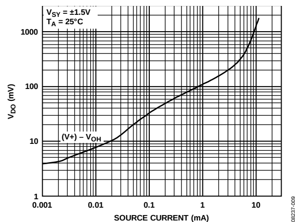
Figure 14. Dropout Voltage vs. Source Current
