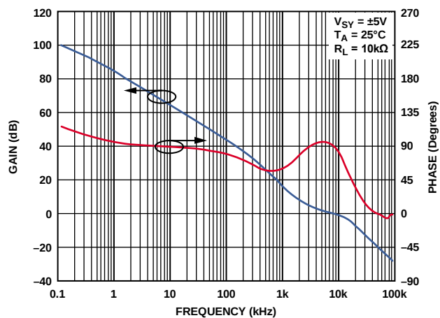
Figure 44. Open-Loop Gain and Phase vs. Frequency
