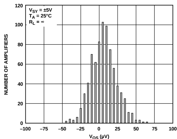
Figure 33. Input Offset Voltage Distribution, SOIC
