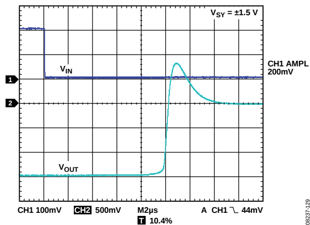
Figure 32. Negative Overload Recovery
