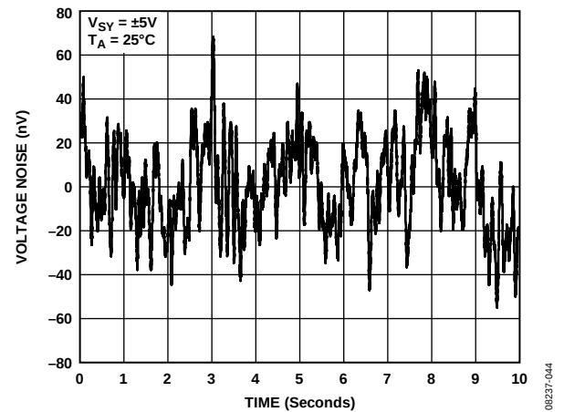
Figure 54. Voltage Noise, 0.1 Hz to 10 Hz
