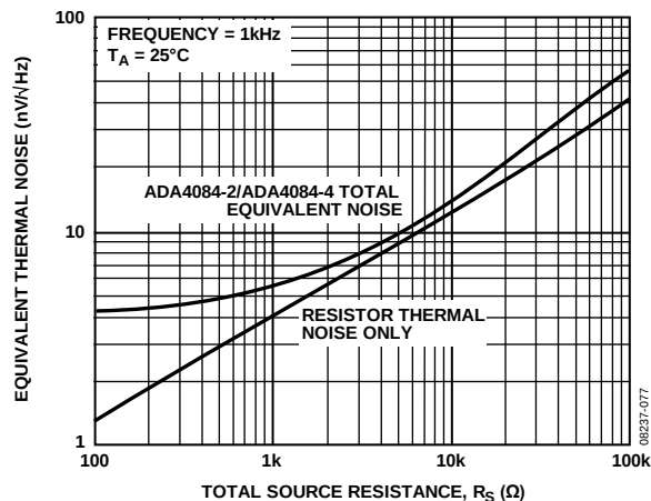
Figure 96. Equivalent Thermal Noise vs. Total Source Resistance
