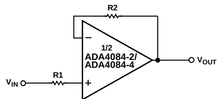
Figure 94. Resistance in Series with Input Limits Overvoltage Currents to Safe Values
