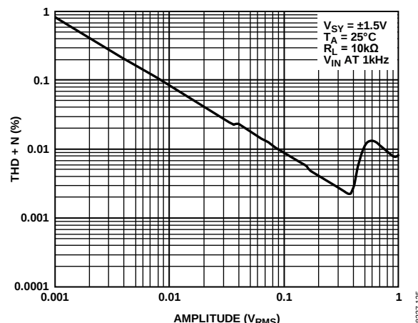
Figure 28. THD + N vs. Amplitude
