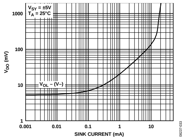
Figure 43. Dropout Voltage vs. Sink Current
