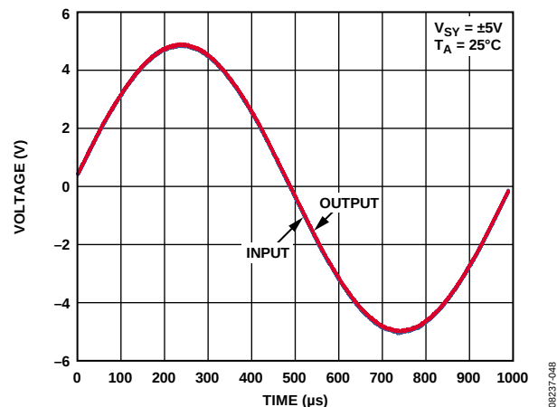
Figure 58. No Phase Reversal
