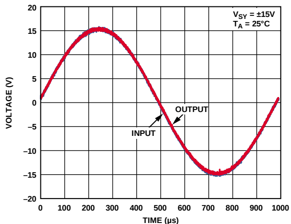
Figure 86. No Phase Reversal
