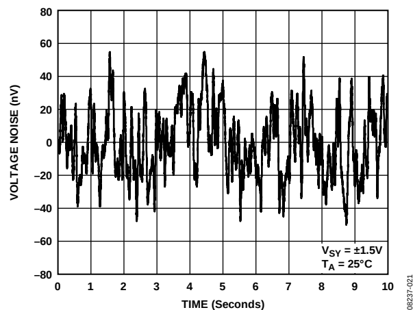
Figure 26. Voltage Noise, 0.1 Hz to 10 Hz
