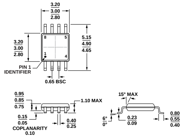
Figure 98. 8-Lead Mini Small Outline Package [MSOP] (RM-8)
