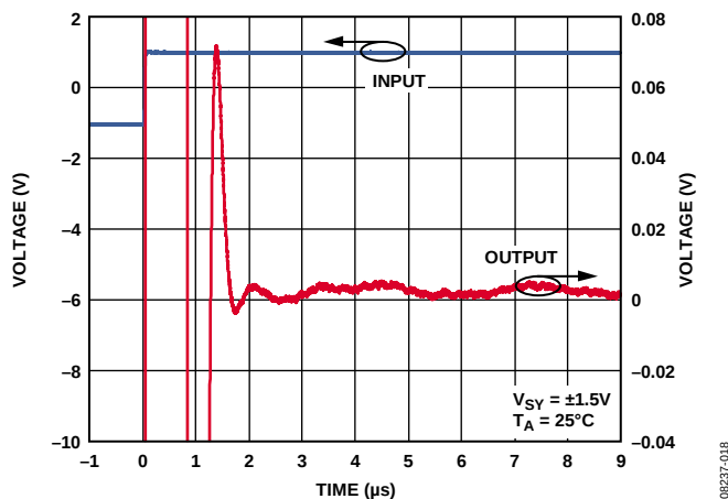
Figure 23. Settling Time
