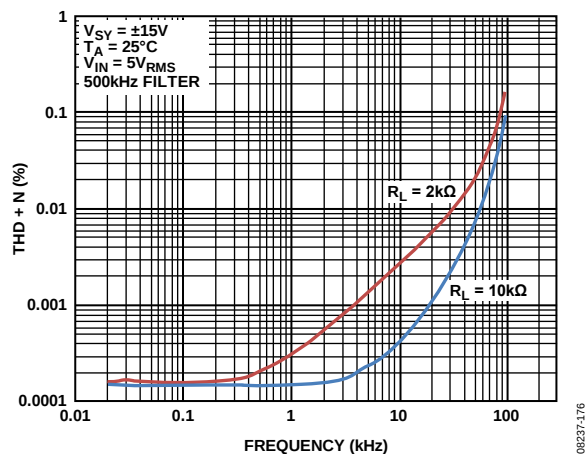
Figure 85. THD + N vs. Frequency
