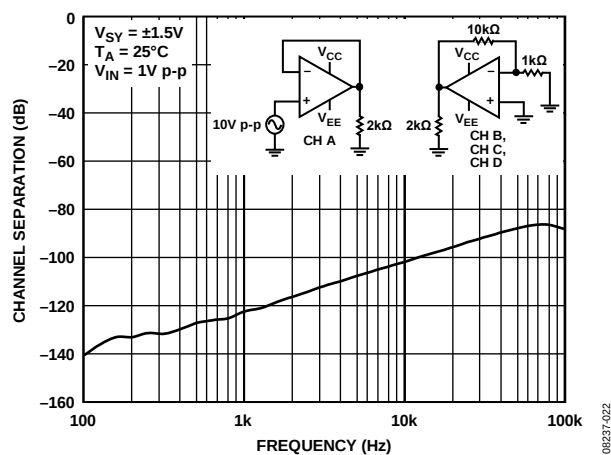
Figure 27. Channel Separation
