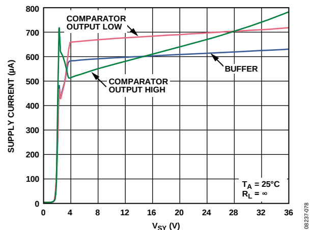
Figure 97. Supply Current vs. Supply Voltage
