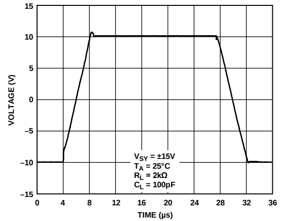
Figure 77. Large Signal Transient Response
