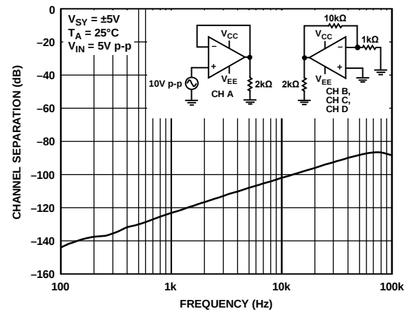
Figure 55. Channel Separation
