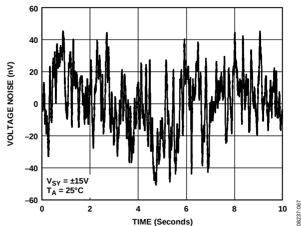
Figure 82. Voltage Noise 0.1 Hz to 10 Hz
