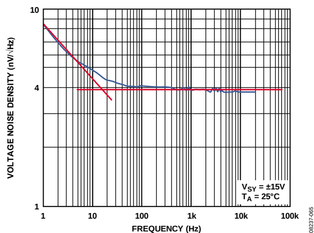
Figure 80. Voltage Noise Density
