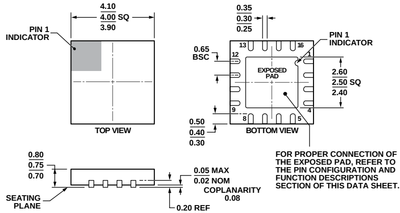
Figure 102. 16-Lead Lead Frame Chip Scale Package [LFCSP_WQ] 4 mm x 4 mm Body, Very Very Thin Quad (CP-16-26) Dimensions shown in millimeters
