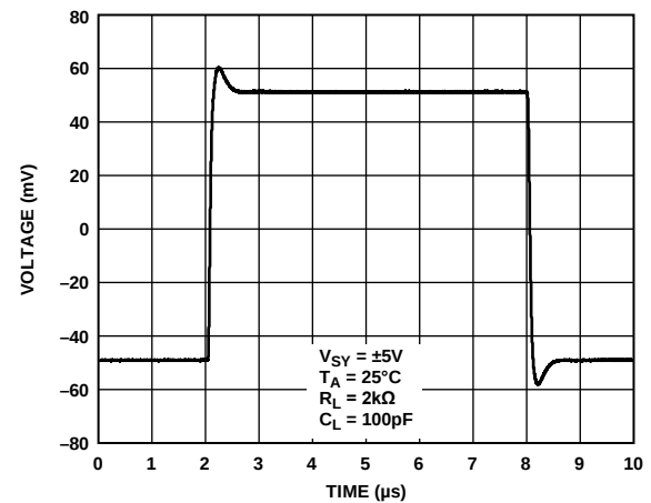
Figure 50. Small Signal Transient Response
