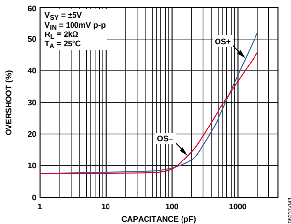
Figure 53. Overshoot vs. Load Capacitance
