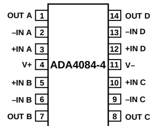
Figure 2. 14-Lead TSSOP (RU)
