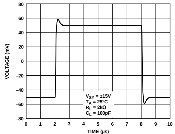
Figure 78. Small Signal Transient Response
