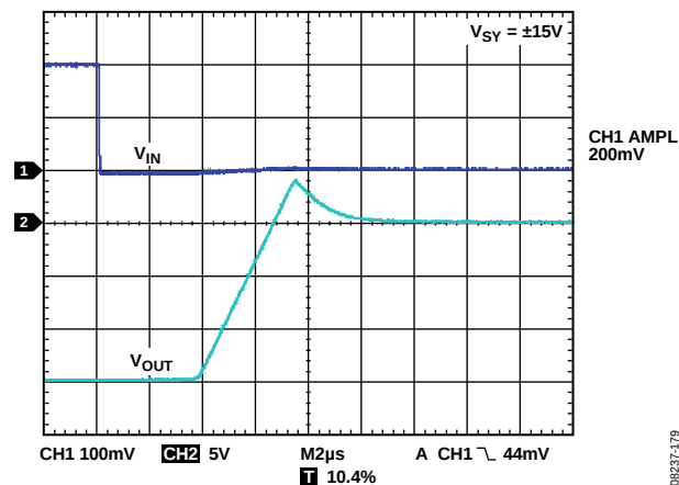
Figure 88. Negative Overload Recovery
