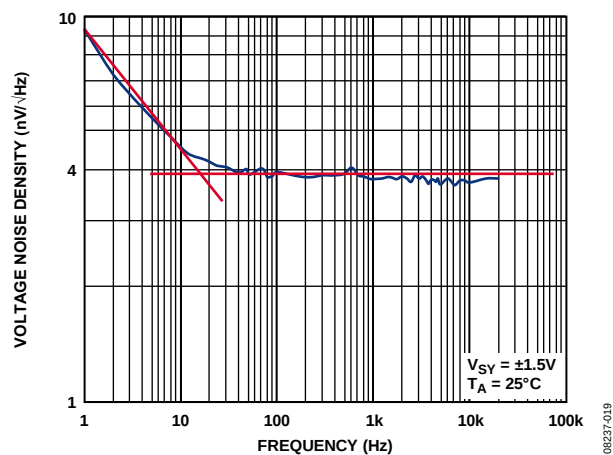
Figure 24. Voltage Noise Density
