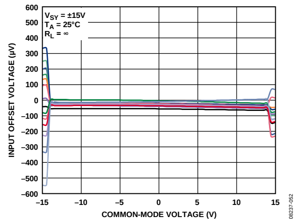
Figure 66. Input Offset Voltage vs. Common-Mode Voltage
