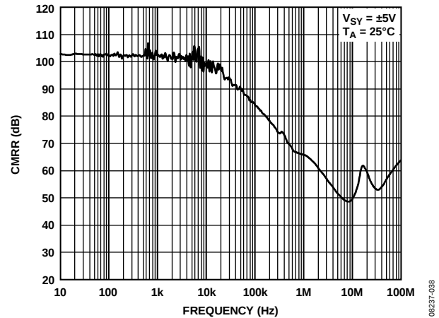
Figure 48. CMRR vs. Frequency
