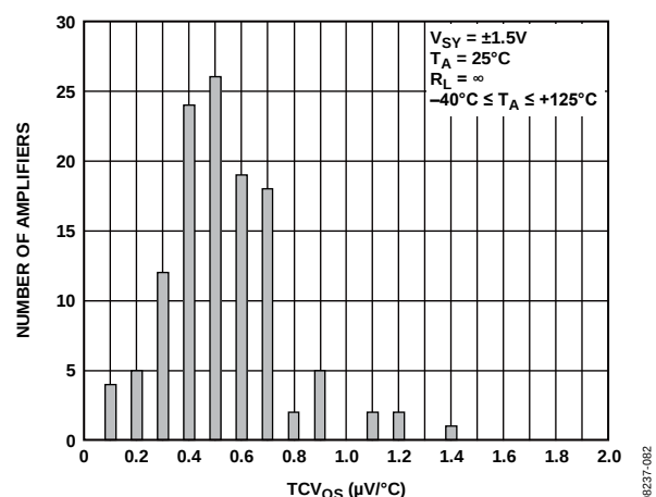
Figure 9. TCV_{OS} Distribution, LFCSP
