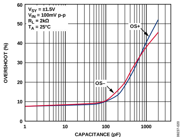
Figure 25. Overshoot vs. Load Capacitance
