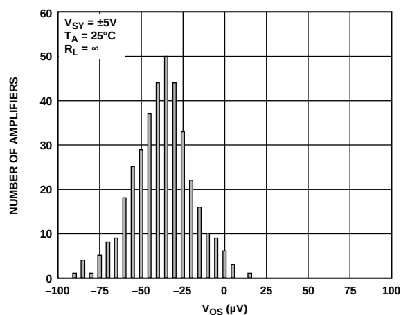
Figure 34. Input Offset Voltage Distribution, MSOP
