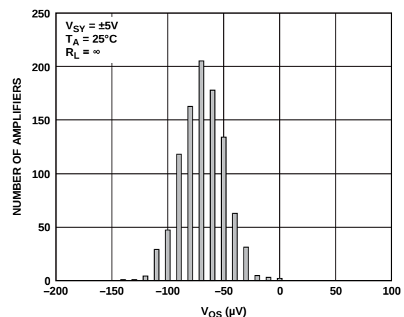
Figure 35. Input Offset Voltage Distribution, ADA4084-2 LFCSP
