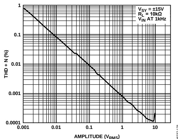
Figure 84. THD + N vs. Amplitude
