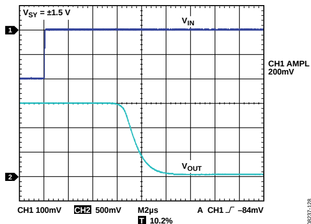
Figure 31. Positive Overload Recovery
