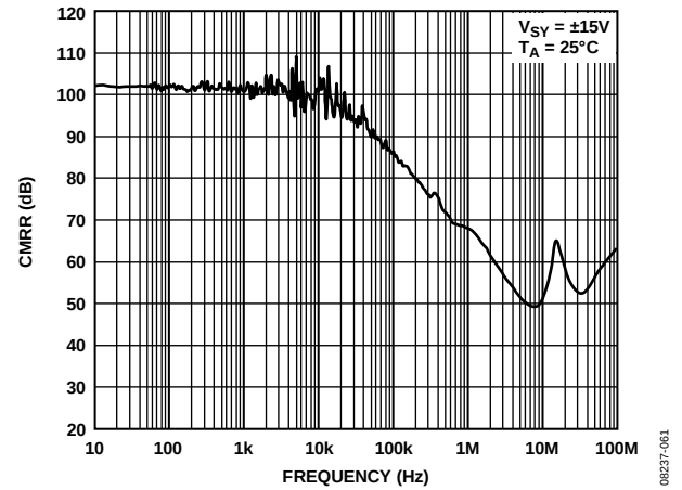
Figure 76. CMRR vs. Frequency
