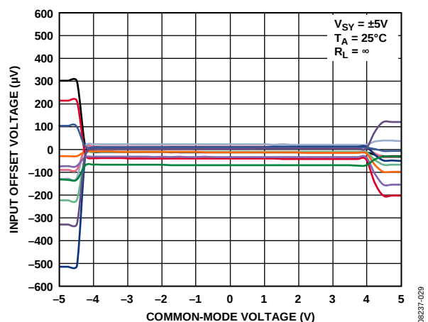
Figure 38. Input Offset Voltage vs. Common-Mode Voltage
