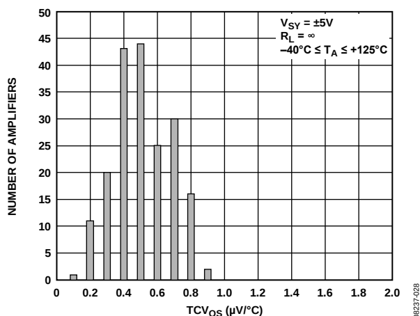
Figure 36. TCV_{OS} Distribution, SOIC and MSOP
