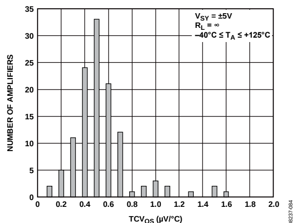
Figure 37. TCV_{OS} Distribution, ADA4084-2 LFCSP
