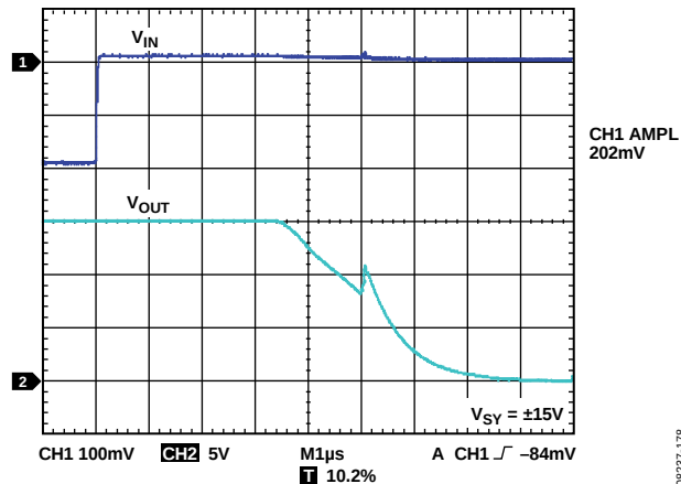
Figure 87. Positive Overload Recovery
