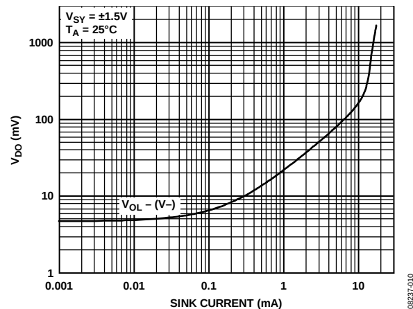
Figure 15. Dropout Voltage vs. Sink Current
