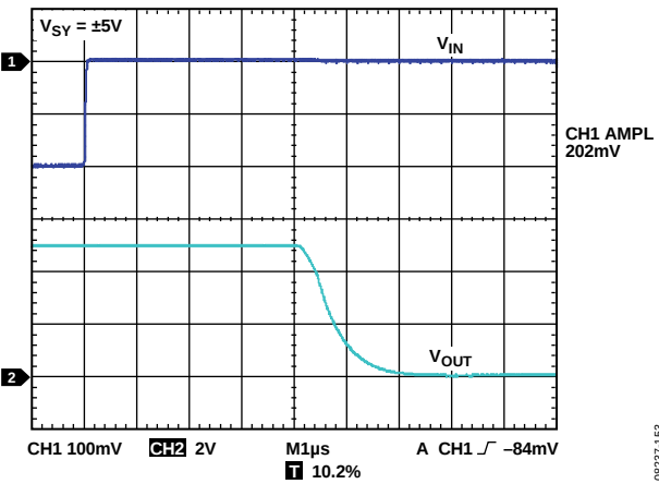
Figure 59. Positive Overload Recovery
