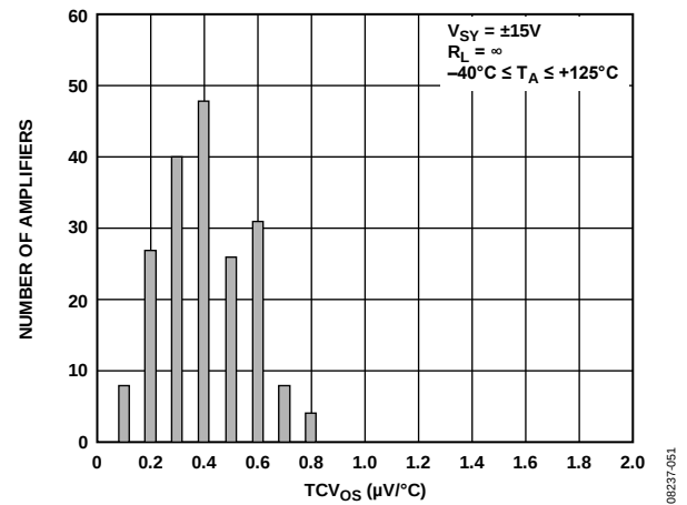
Figure 64. TCV_{OS} Distribution, SOIC and MSOP
