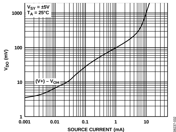
Figure 42. Dropout Voltage vs. Source Current
