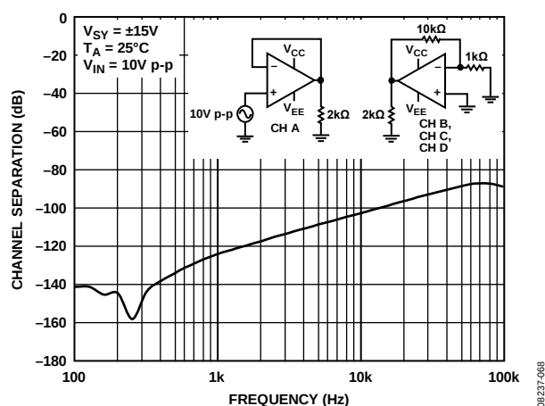
Figure 83. Channel Separation
