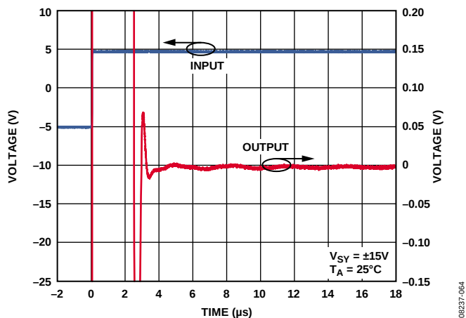
Figure 79. Settling Time
