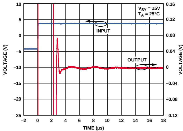
Figure 51. Settling Time
