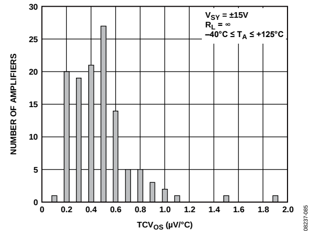
Figure 65. TCV_{OS} Distribution, ADA4084-2 LFCSP
