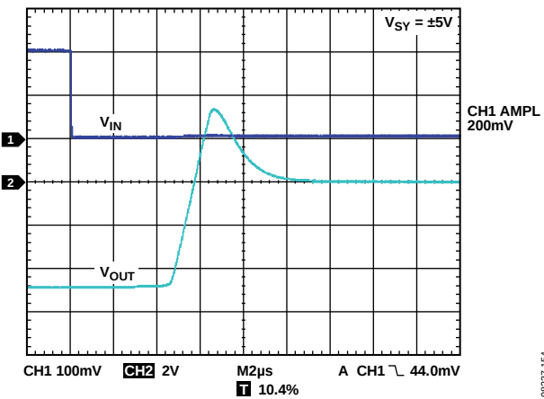
Figure 60. Negative Overload Recovery
