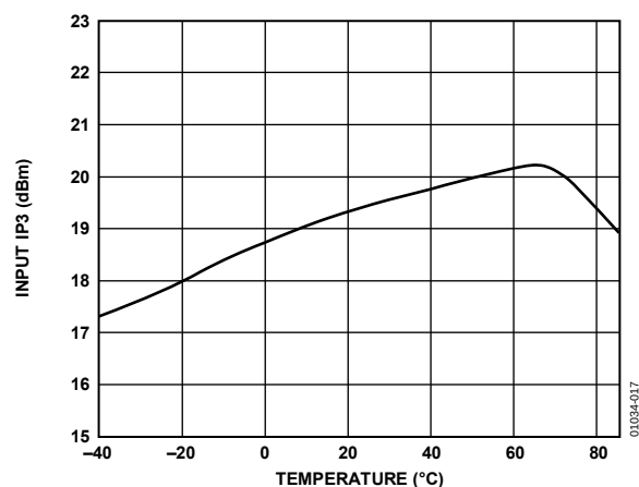
Figure 17. Input IP3 Performance Over Temperature; f_{IN} = 900 MHz, f_{OUT} = 170 MHz
