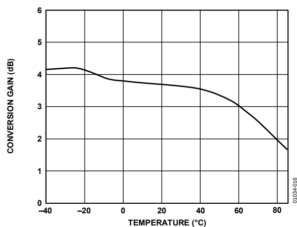
Figure 16. Gain Performance Over Temperature; f_{IN} = 900 MHz, f_{OUT} = 170 MHz
