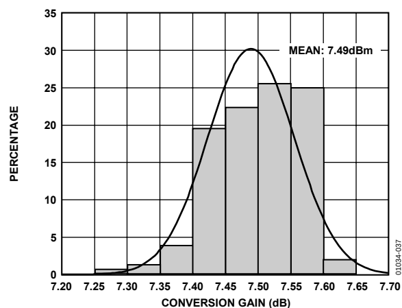
Figure 37. Gain Histogram; f_{IN} = 150 MHz, f_{OUT} = 900 MHz
