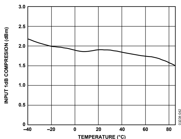
Figure 42. Input 1dB Compression Point Performance Over Temperature; f_{IN} = 150 MHz, f_{OUT} = 900 MHz
