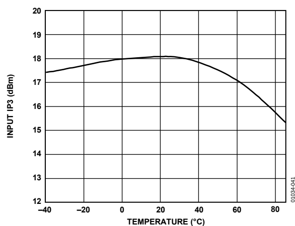
Figure 41. Input IP3 Performance Over Temperature; f_{IN} = 150 MHz, f_{OUT} = 900 MHz
