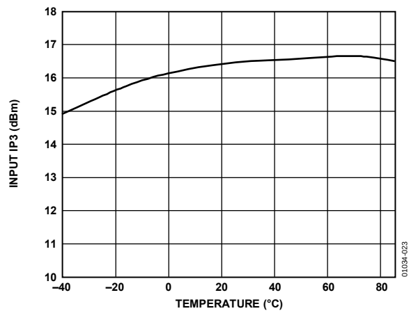
Figure 23. Input IP3 Performance Over Temperature; f_{IN} = 1900 \text{ MHz} , f_{OUT} = 170 \text{ MHz}
