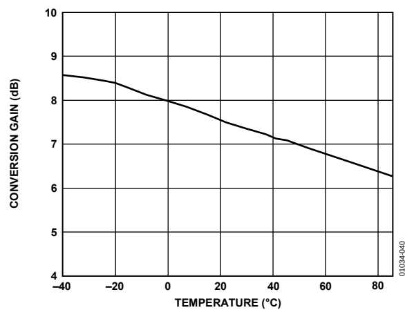
Figure 40. Gain Performance Over Temperature; f_{IN} = 150 MHz, f_{OUT} = 900 MHz
