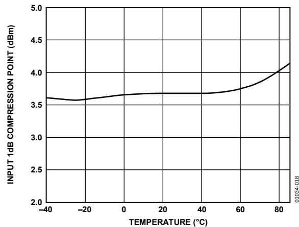
Figure 18. Input 1dB Compression Point Performance Over Temperature; f_{IN} = 900 MHz, f_{OUT} = 170 MHz
