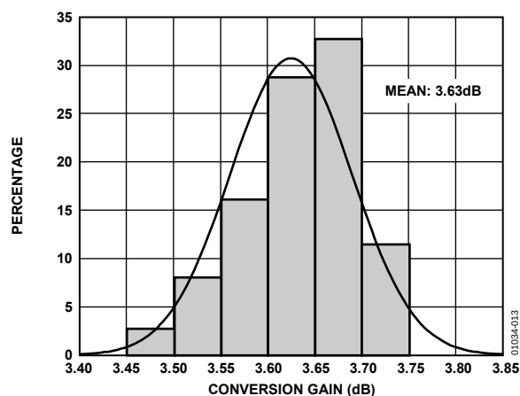
Figure 13. Gain Histogram; f_{IN} = 900 MHz, f_{OUT} = 170 MHz
