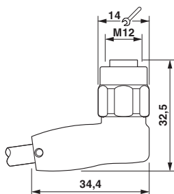
Dimensioned drawing
