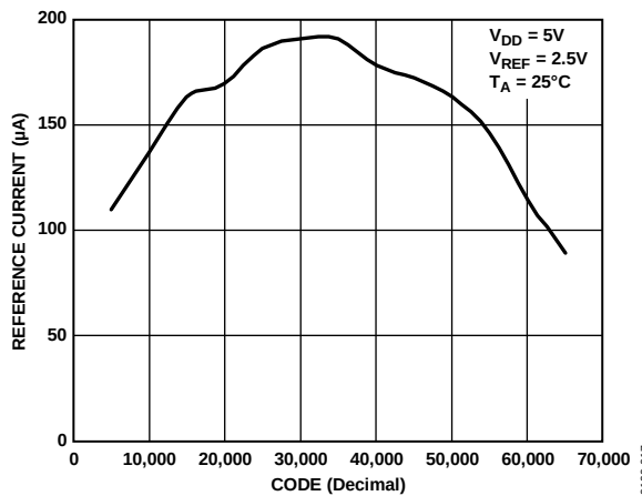
Figure 18. AD5512A/AD5542A Reference Current vs. Code
