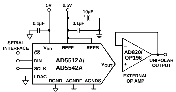
Figure 31. Unipolar Output
