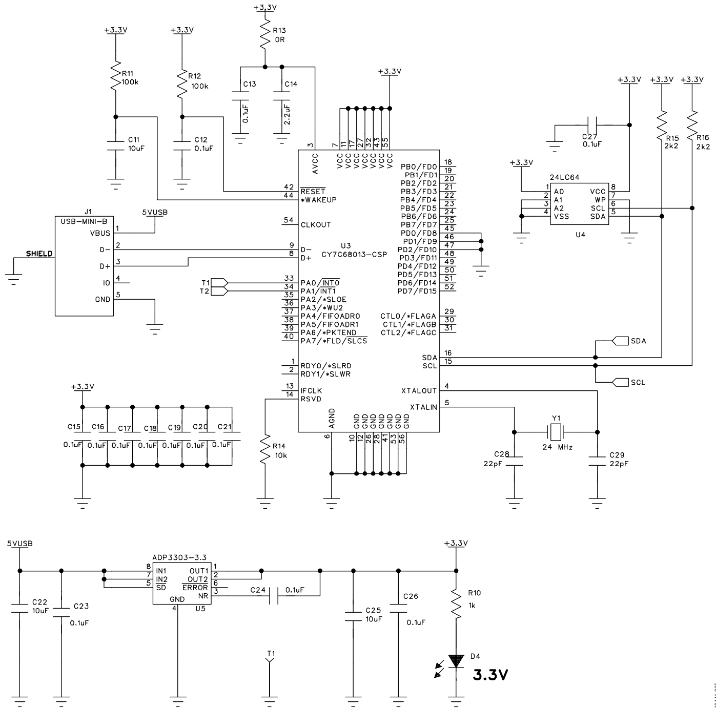
Figure 32. EVAL-AD5933EBZ Schematic
