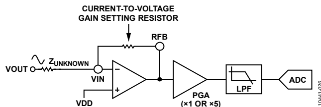
Figure 25. AD5933 System Voltage Gain
