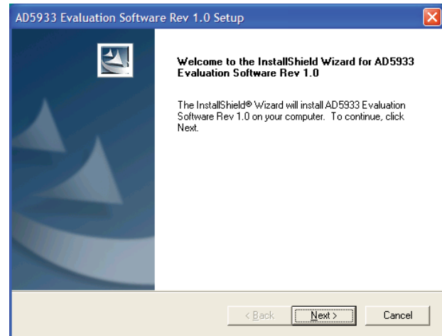
Figure 3. Installation Wizard
