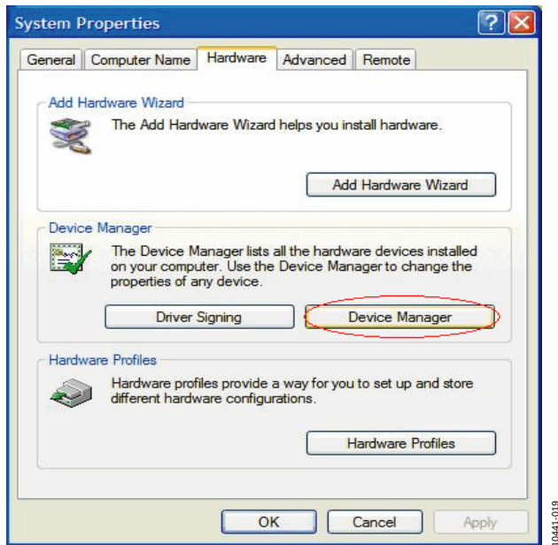
Figure 18. System Properties
