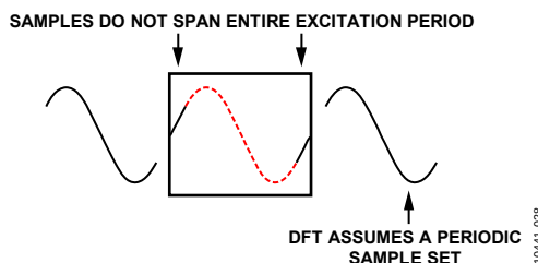
Figure 27. Sample Set Not Spanning the Entire Excitation Period
