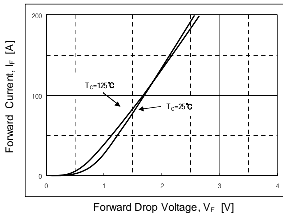
Fig 15. Forward characteristics
