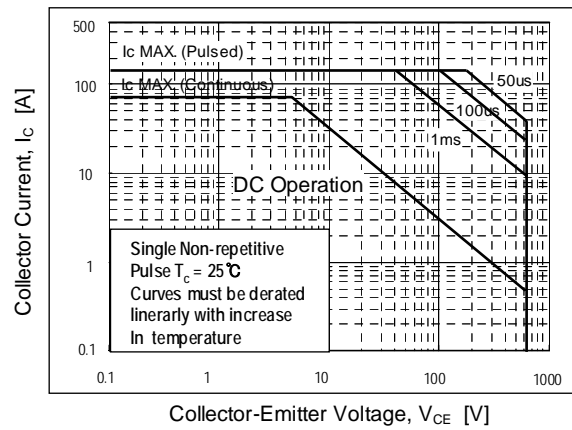
Fig14. SOA characteristics
