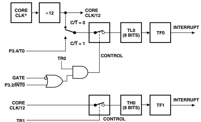
Figure 37. Timer/Counter 0, Mode 3
