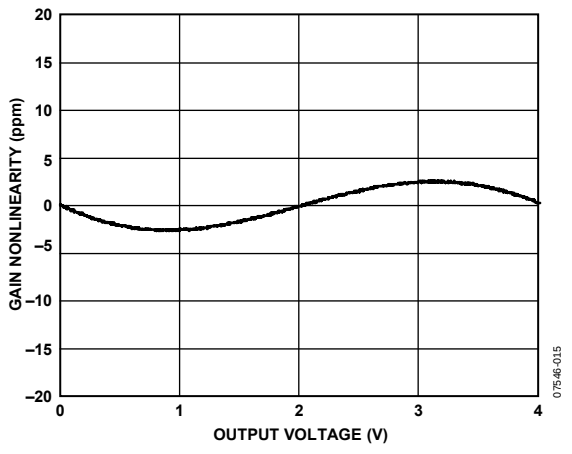
Figure 16. Gain Nonlinearity, R_L = 600\ \Omega , 2\ k\Omega , 10\ k\Omega
