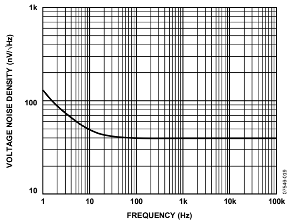
Figure 21. Voltage Noise Density vs. Frequency, Referred to Output
