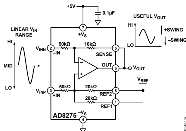
Figure 37. Shared Reference
