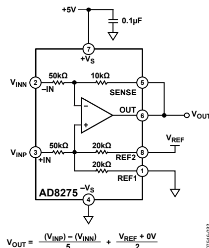
Figure 34. Basic Configuration 2: Split Reference
