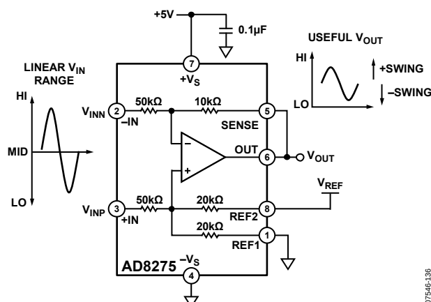
Figure 36. Split Reference
