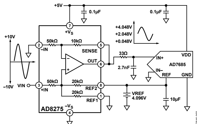
Figure 2. Translating \pm 10 V to 4.096 V ADC Full Scale
