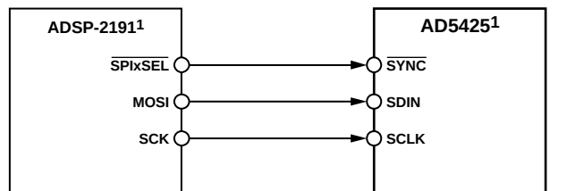
Figure 38. ADSP-2191 SPI-to-AD5425 Interface
