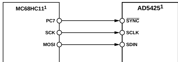
Figure 43. 68HC11/68L11-to-AD5425 Interface
