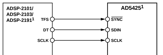
Figure 39. ADSP-2101/ADSP-2103/ADSP-2191 SPORT-to-AD5425 Interface
