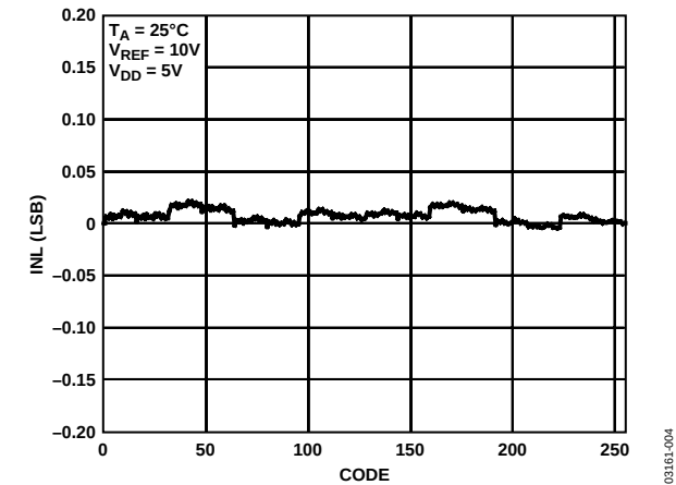
Figure 4. INL vs. Code (8-Bit DAC)
