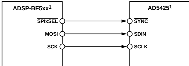
Figure 40. ADSP-BF5xx-to-AD5425 Interface
