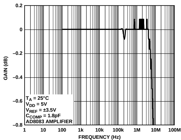
Figure 18. Reference Multiplying Bandwidth—All 1s Loaded
