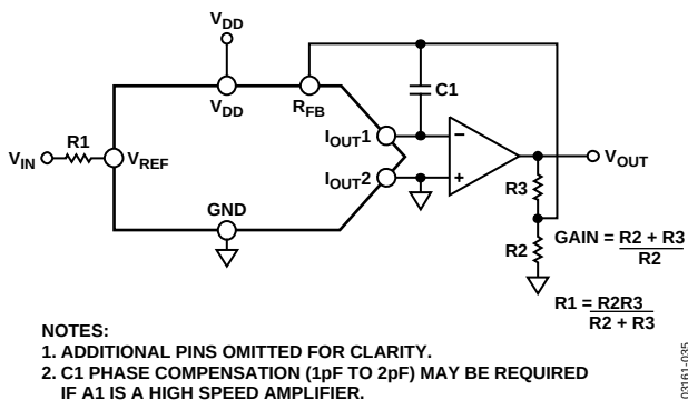
Figure 35. Increasing the Gain of Current Output DAC
